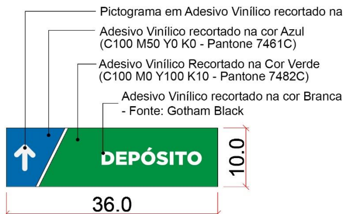
LAYOUT PLACA INDIVIDUAL
